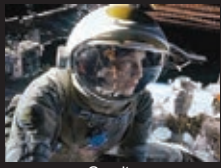
Gravity
